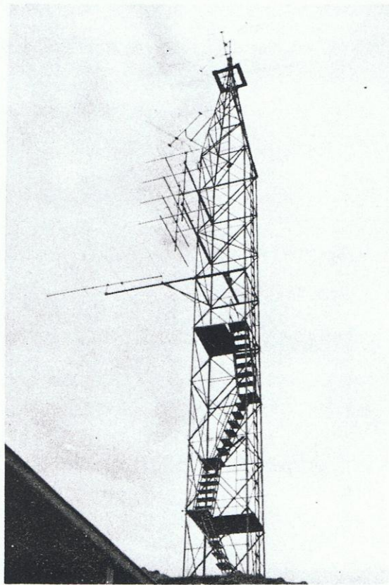
TV DX Antenna Array—George Palmer, Victoria, Australia
