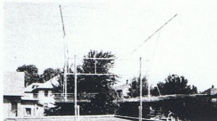
Model No. 94-HD 32-element Quad VHF Lo-Band
