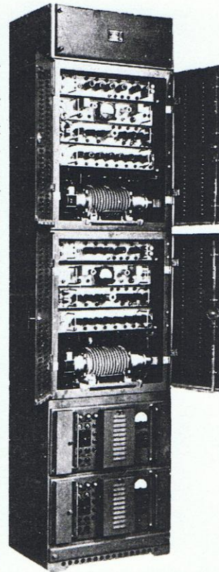
One rack of Microwave Receiving-Transmitting Equipment . . . a la Moscow! This rack holds two "Trunk Units," each capable of receiving and transmitting 600 telephone conversations, or one television channel. Power supply units are on the bottom.
