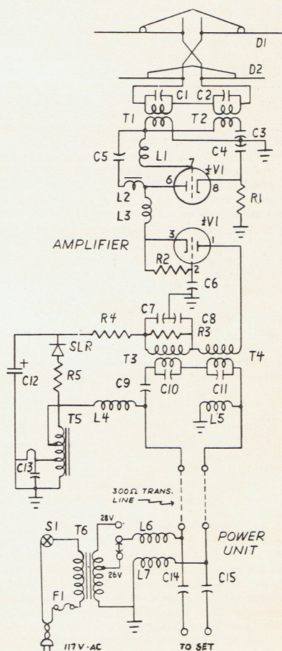
Winegard Powertron Schematic. (Courtesy Winegard)
