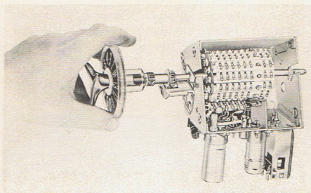
Zenith Gold Video Guard Turret Tuner
