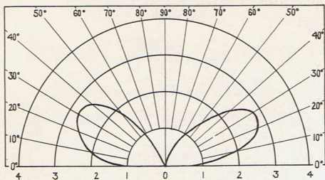
One-quarter wave length (at any frequency) above ground . . . pattern shows maximum antenna gain for signals returning at high radiation angles (20-40 degrees).
