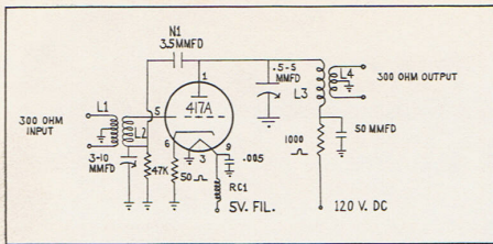
The Wright Circuit
