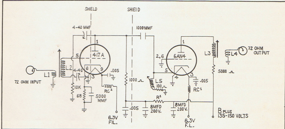
North Bay 417A-6AN4 Pre-Amp
