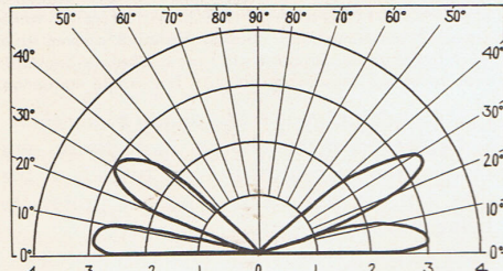
One full wave above ground . . . (at any frequency) the antenna now works best at the lower angles of radiation.
