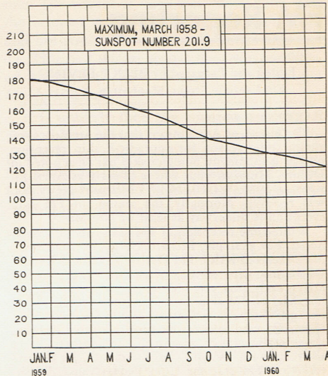
Declining Sun Spots - to April 1960
