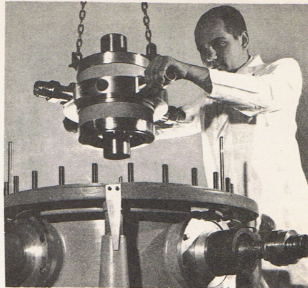
RCA technician Gerald Grill lowers the world's most powerful tube into a test chamber at the RCA ELECTRON TUBE PLANT in Lancaster, Pa. This 150 pound monster tube is capable of 5,000,000 watts peak power (long pulse) on frequencies to 450 megacycles. Its importance may soon be demonstrated when it is put to use in super high power scatter circuits which are destined to be the forerunner to intercontinental TV. (Photo courtesy of RCA Electronic Age)
