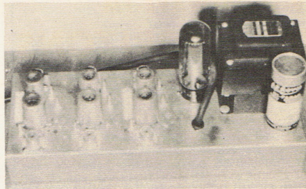
3 Channel 417A Pre-Amp by Hosken, North Bay
