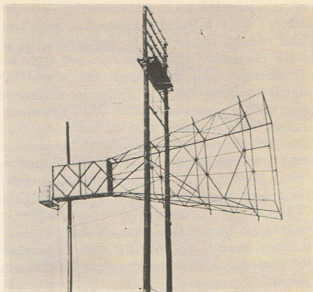
Experimental horn antenna during installation several years ago at the Muscle Shoals, Ala. CATV system. An early, and still operating, design to reject interfering signals.
