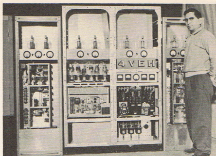
This "proud gentleman" is M. E. (Mardy) Picazo, Station Manager and Chief Engineer, 4VEH, "The Evangelical Voice of the West Indies," Cap Haitien, Haiti. He is shown in Elkhart, Indiana, with the TWO new 2.5-kW transmitters of 4VEH which were built in the shop of the International Radio and Electronics Corporation. By now one of the NEW transmitters should be operating as 4VEH on 6.100. Reception reports are desired.
