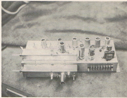
UHF-TR-10 Multiplier String
