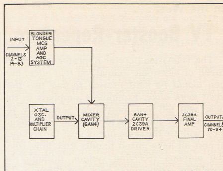
Eitel UHF-TR-10 Block Diagram
