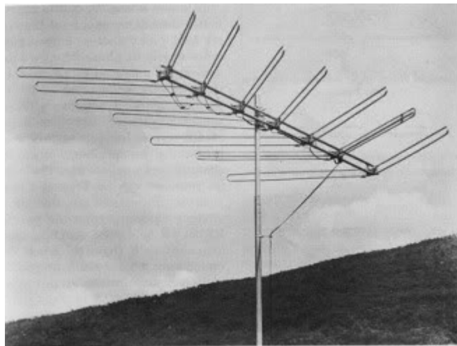
Fig. 3-26. The traveling-wave antenna. (Courtesy of Channel Master Corp.)
